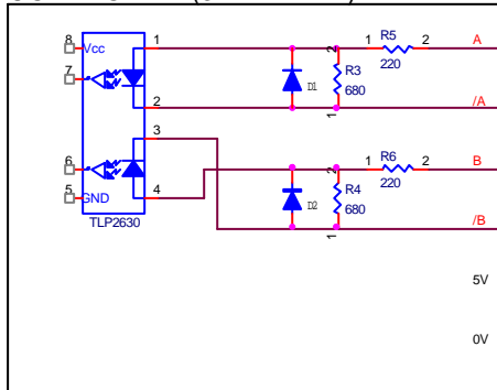
CONTROLLER(34 )
